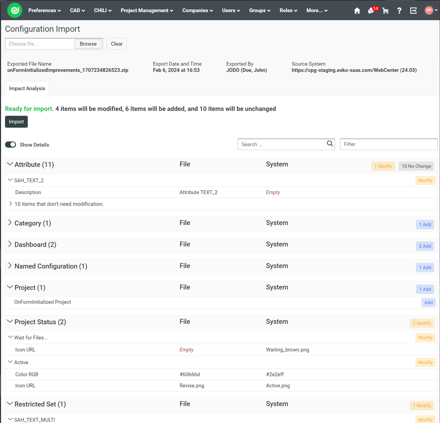
Sample configuration import UI
